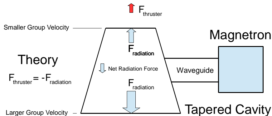
Figure 1. EMDrive Concept.
